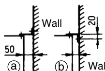
Space required for service (In case of right side piping)
