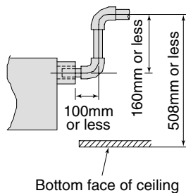
Space required for installation and servicing
