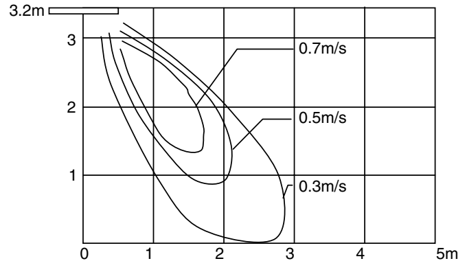
MMU-AP0151MH, MMU-AP0181MH (High ceiling mode)
