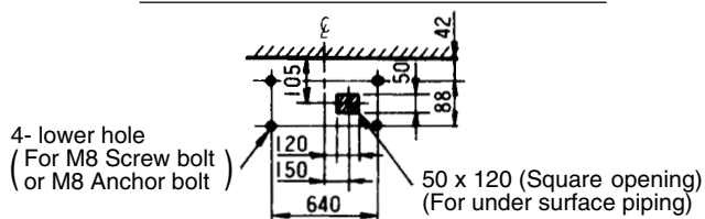
Details of hole for lower side piping
