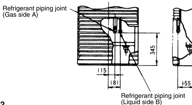
Details of hole for lower side piping
