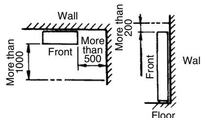
Space required for service (In case of right side piping)
