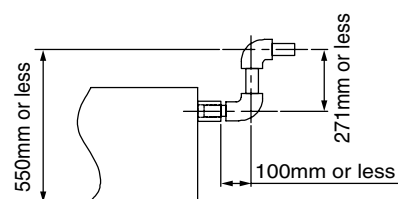
Drain-up piping
